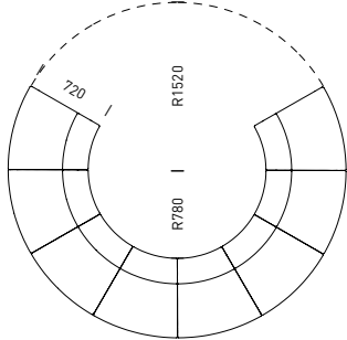
Convex modular lounge
