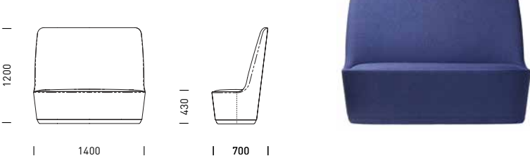
Double High Back Lounge
